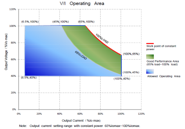
V/I Curve
