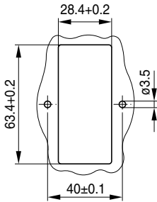
Mounting holes for Mounting version II
