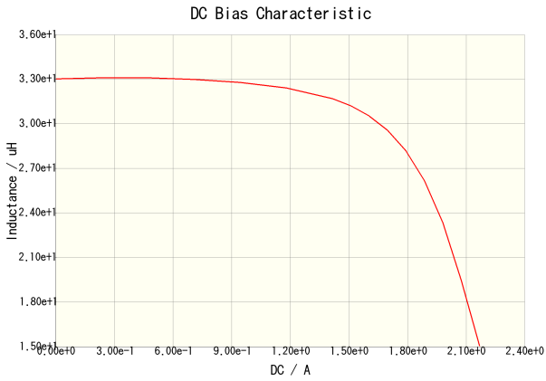
CLF7045T-330M(Amb. Temp. = 20degc)
