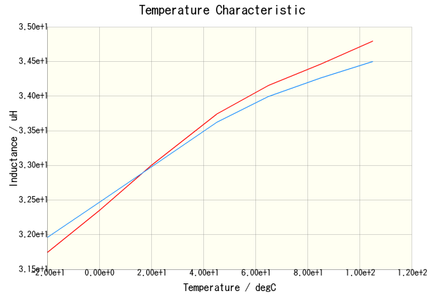
CLF7045T-330M(DC = 0A)
