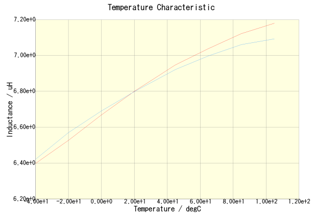
CLF6045T-6R8N(DC = 0A)
