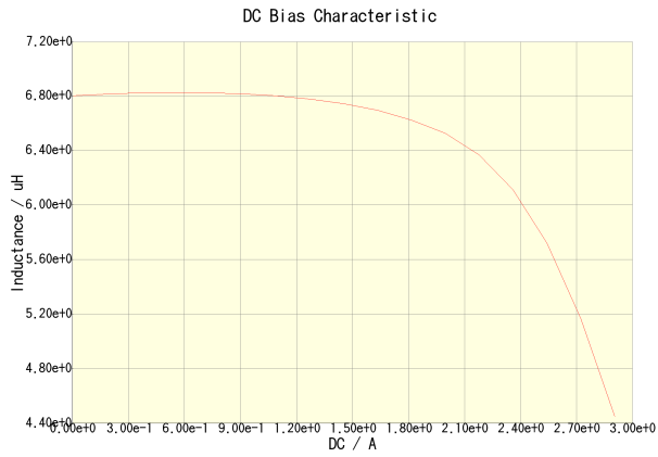
CLF6045T-6R8N(Amb. Temp. = 20degc)
