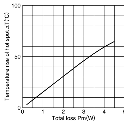
Temperature rise vs. Total loss for ETD39 core (Typical) (Ambient temperature: 25°C)
