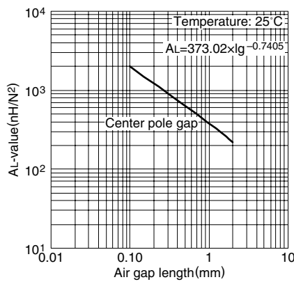
AL-value vs. Air gap length for PC47EE60 core (Typical)
