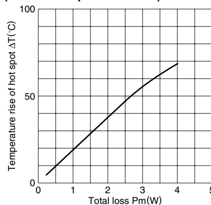
Temperature rise vs. Total loss for ETD34 core (Typical) (Ambient temperature: 25°C)
