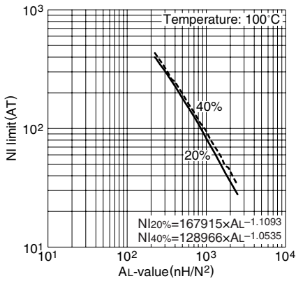
NI limit vs. AL-value for PC47EE60 gapped core (Typical)
