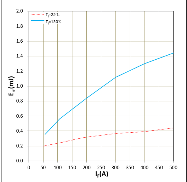
Figure 19. E_{rr} vs I_F V_{DD} = 600\text{V} , R_G = 4.5\Omega , V_{GS} = +15\text{V}/-4\text{V} Inductive Load
