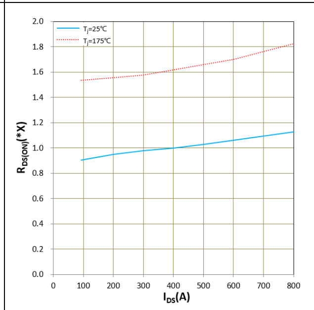
Figure 11. R_{DS(ON)} vs I_{DS} 1.0x = 4.2\text{m}\Omega
