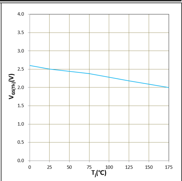
Figure 13. V_{GS(th)} vs T_j V_{GS} = V_{DS} , I_D = 110\text{mA}
