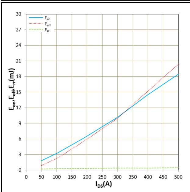
Figure 16. E_{on} , E_{off} , E_{rr} vs I_{DS} T_j = 25^\circ\text{C} , V_{CC} = 600\text{V} , R_G = 4.5\Omega , V_{GS} = +15\text{V}/-4\text{V} Inductive Load
