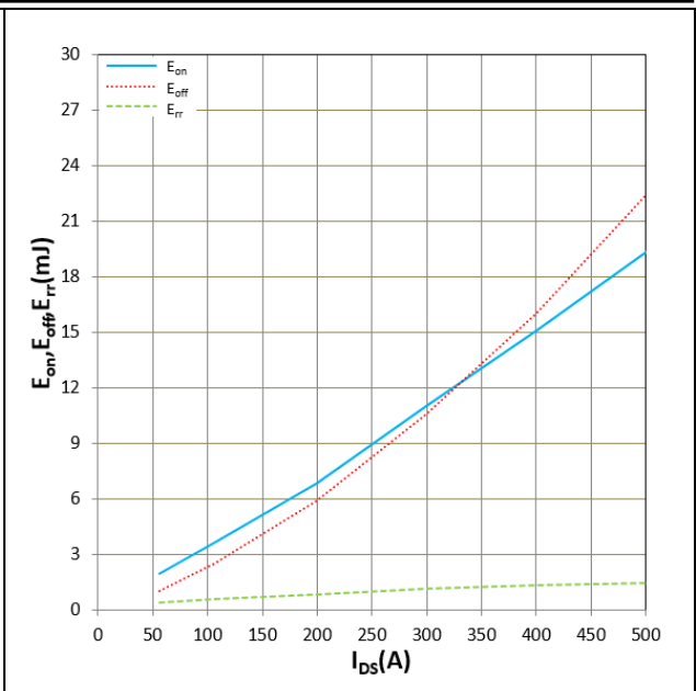
Figure 17. E_{on} , E_{off} , E_{rr} vs I_{DS} T_j = 150^\circ\text{C} , V_{CC} = 600\text{V} , R_G = 4.5\Omega , V_{GS} = +15\text{V}/-4\text{V} Inductive Load
