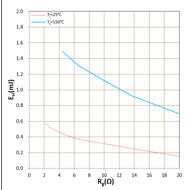
Figure 18. E_{rr} vs R_G V_{DD} = 600\text{V} , I_F = 400\text{A} , V_{GS} = +15\text{V}/-4\text{V} Inductive Load
