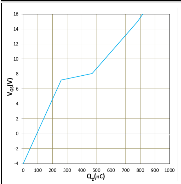
Figure 12. V_{GS} vs Q_g T_j = 25^\circ\text{C} , V_{CC} = 800\text{V} , I_D = 400\text{A}
