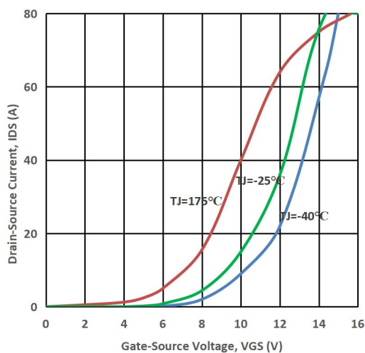
Fig5. Transfer Characteristic
