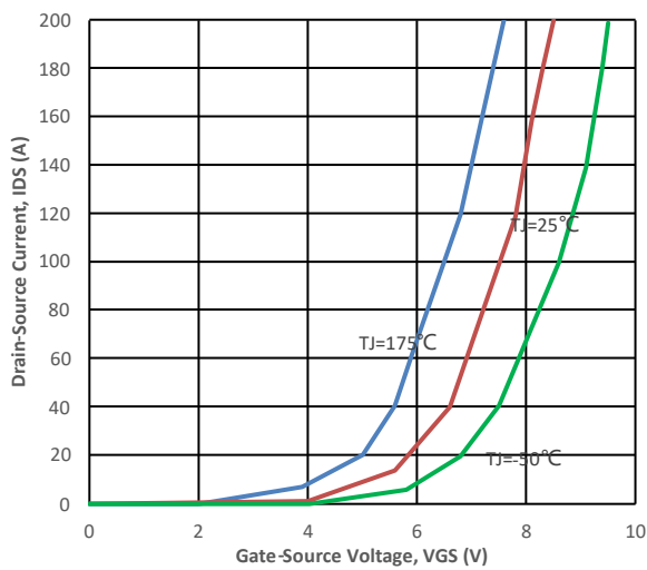
Fig5. Transfer Characteristic
