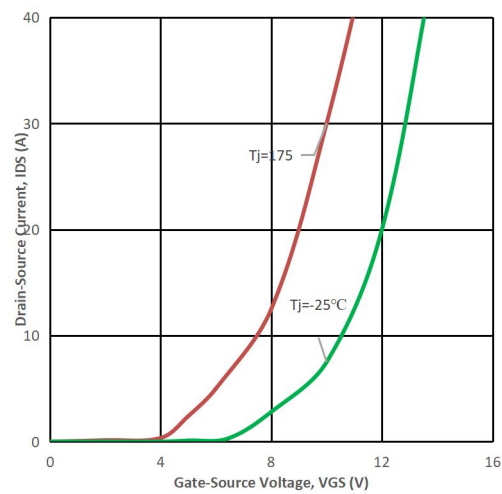
Fig5. Transfer Characteristic
