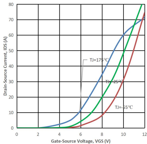
Fig5. Transfer Characteristic
