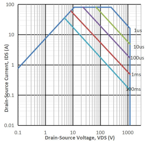
Fig18. Safe Operating Area
