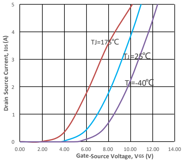
Fig5. Transfer Characteristic
