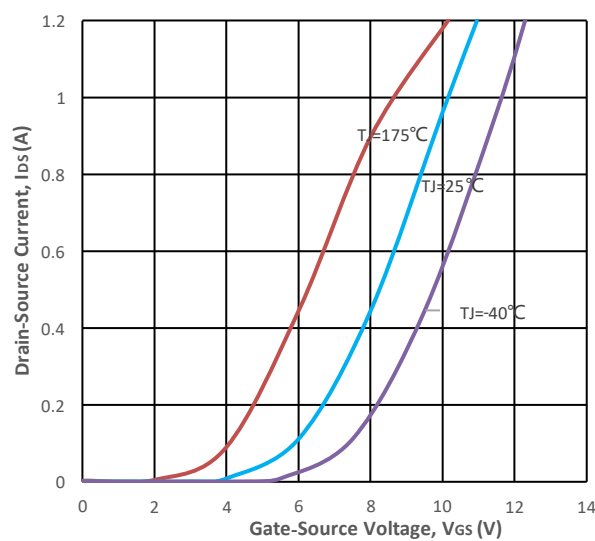
Fig5. Transfer Characteristic
