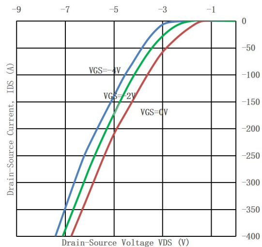
Fig6. Body Diode Characteristic at 25^\circ\text{C}
