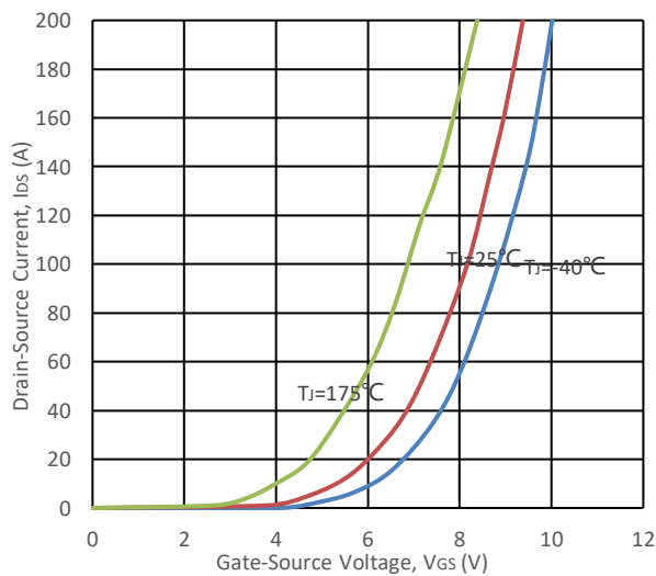
Fig5. Transfer Characteristic
