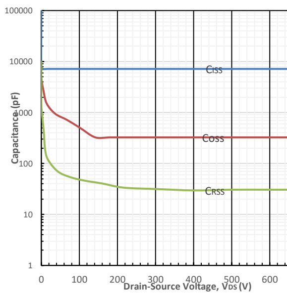
Fig11. Capacitances vs. Drain-Source
