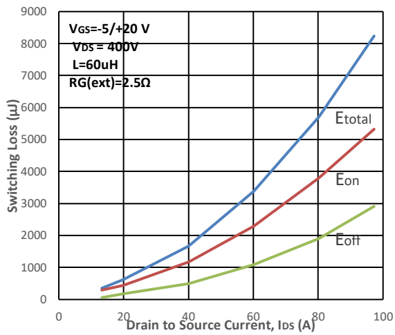
Fig13. Switching Energy vs. Drain Current
