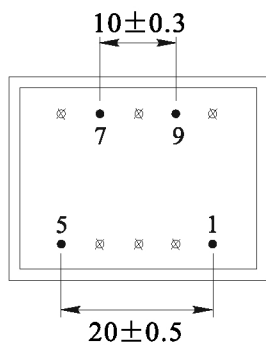
Bottom view
