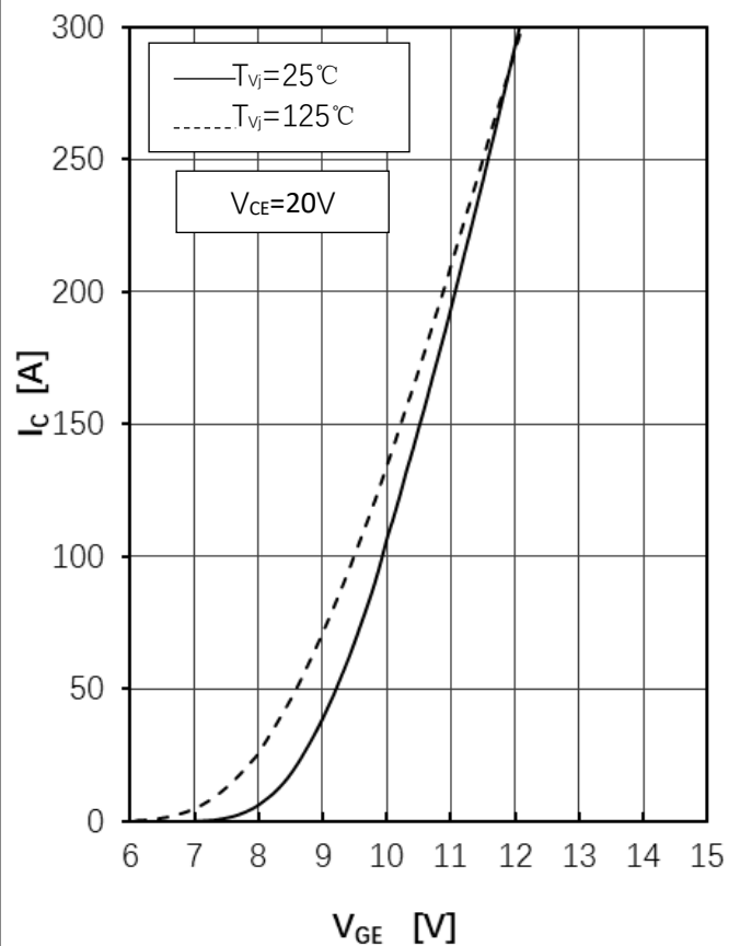
Fig2.IGBT Transfer Characteristics
