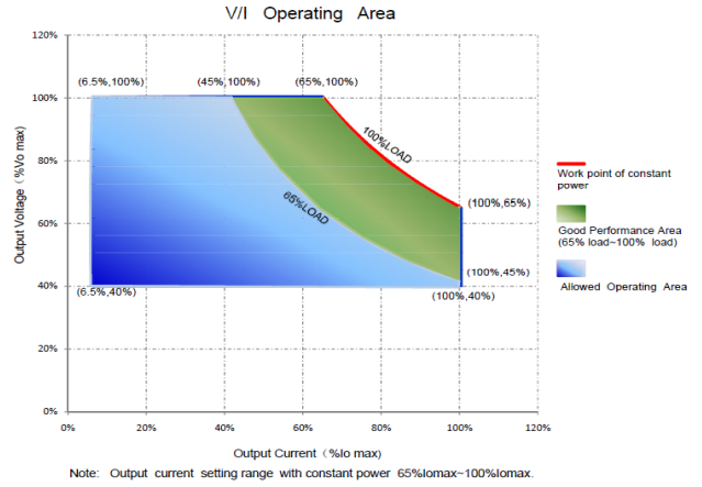
V/I Curve
