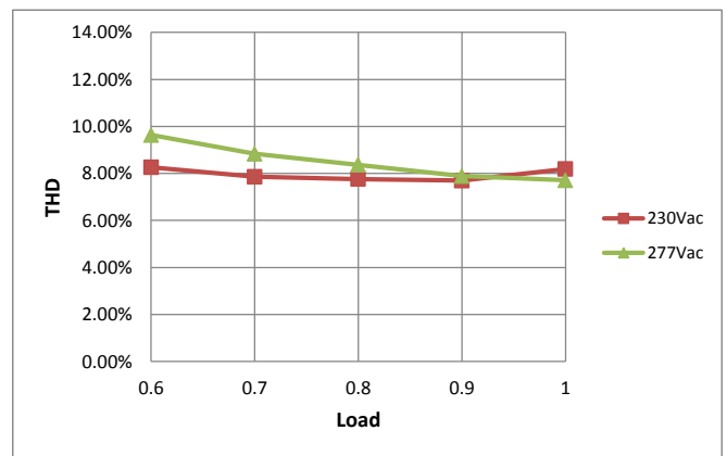
THD Curve
