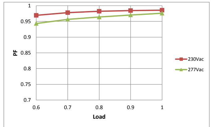
Power Factor Curve
