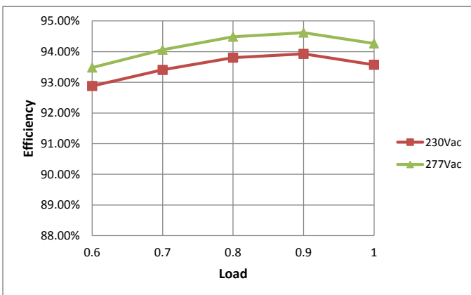
Efficiency VS. Load Curve (Io=4000mA)
