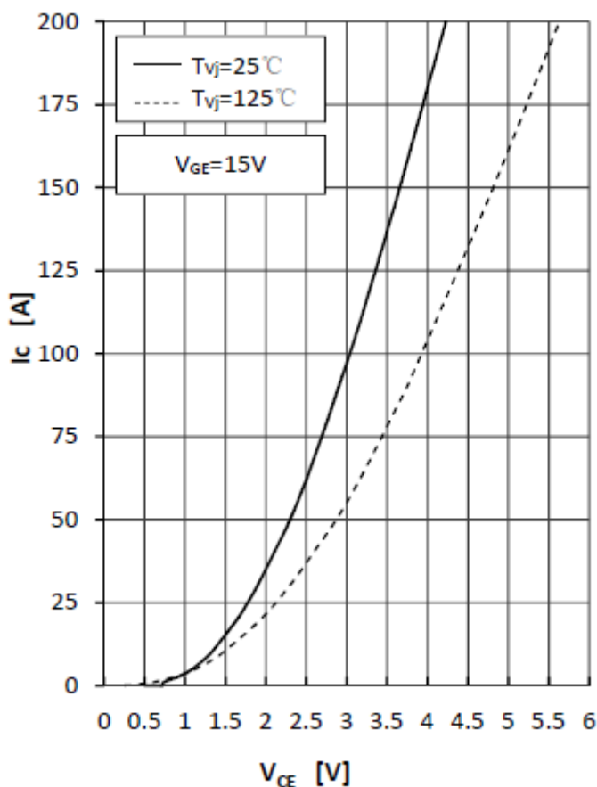
Fig1.IGBT Output Characteristics
