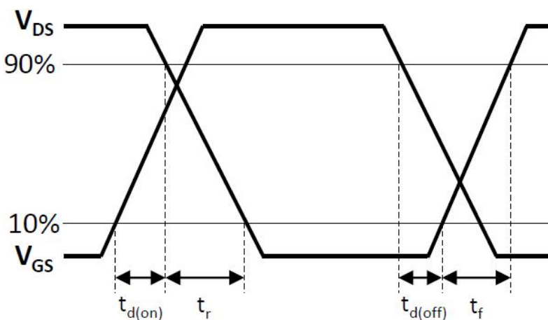
Figure 21. Switching Times Definition
