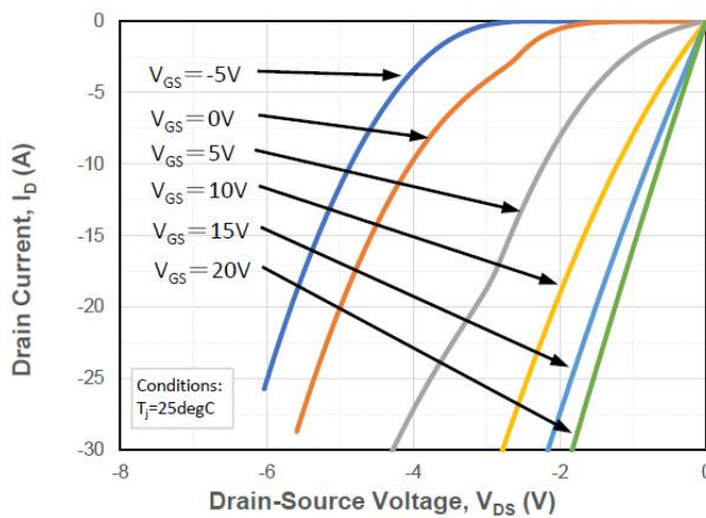
Figure 8. Reverse Output Characteristics at T_j = 25^{\circ}\text{C}
