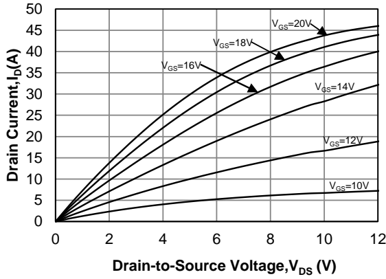
Fig 1. Output Characteristics (T j =-55°C)
