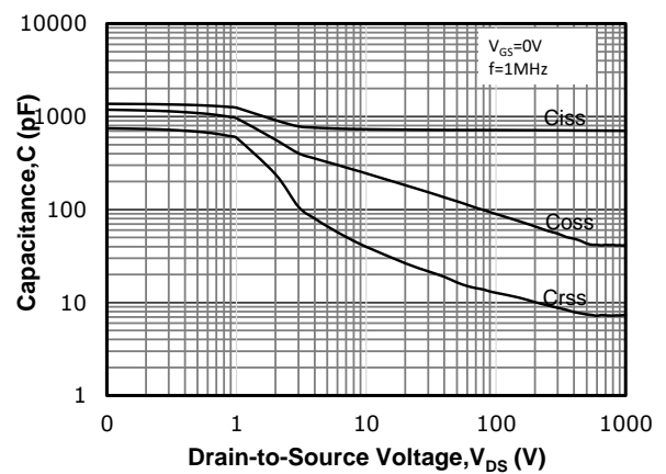
Fig 12: Capacitance Characteristics
