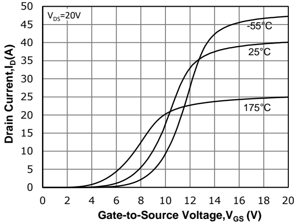
Fig 7: Transfer Characteristics
