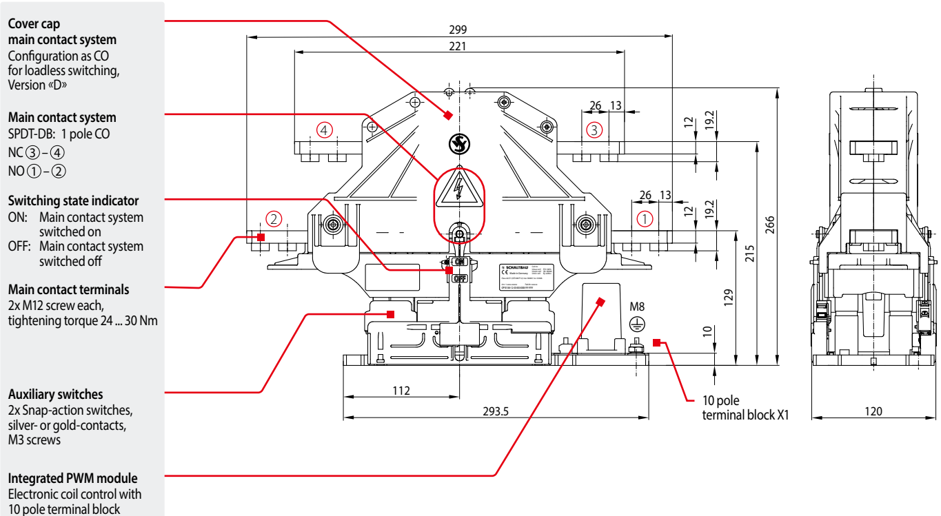
Dimension diagram CP3115-12-D, CP3130-12-D 1 pole SPDT-DB | U_n = 1,500/3,000\text{ V} | I_{th} = 1,200\text{ A} | Breaking capacity: none
