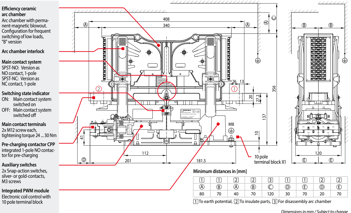
Dimension diagram CP1115-20-B, CP1130-20-B 1 pole SPST-NO | Un = 1,500/3,000 V | Ith = 2,000 A | Breaking capacity: medium CP2115-20-B, CP2130-20-B 1 pole SPST-NC | Un = 1,500/3,000 V | Ith = 2,000 A | Breaking capacity: medium
