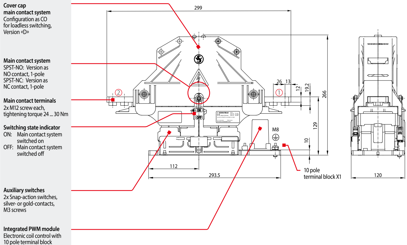
Dimension diagram CP1115-12-D, CP1130-12-D 1 pole SPST-NO | U_n = 1,500/3,000\text{ V} | I_{th} = 1,200\text{ A} | Breaking capacity: none CP2115-12-D, CP2130-12-D 1 pole SPST-NC | U_n = 1,500/3,000\text{ V} | I_{th} = 1,200\text{ A} | Breaking capacity: none
