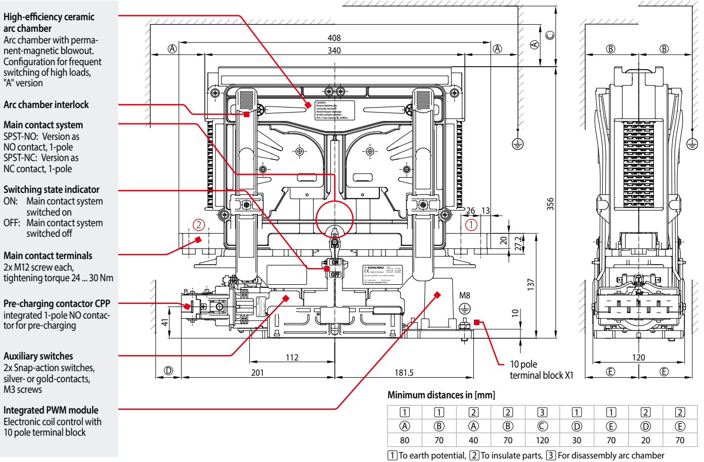
Dimension diagram CP1115-20-B, CP1130-20-B 1 pole SPST-NO | Un = 1,500/3,000 V | Ith = 2,000 A | Breaking capacity: medium CP2115-20-B, CP2130-20-B 1 pole SPST-NC | Un = 1,500/3,000 V | Ith = 2,000 A | Breaking capacity: medium
