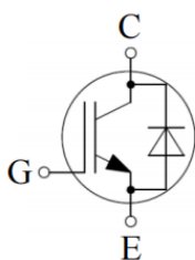
Circuit
